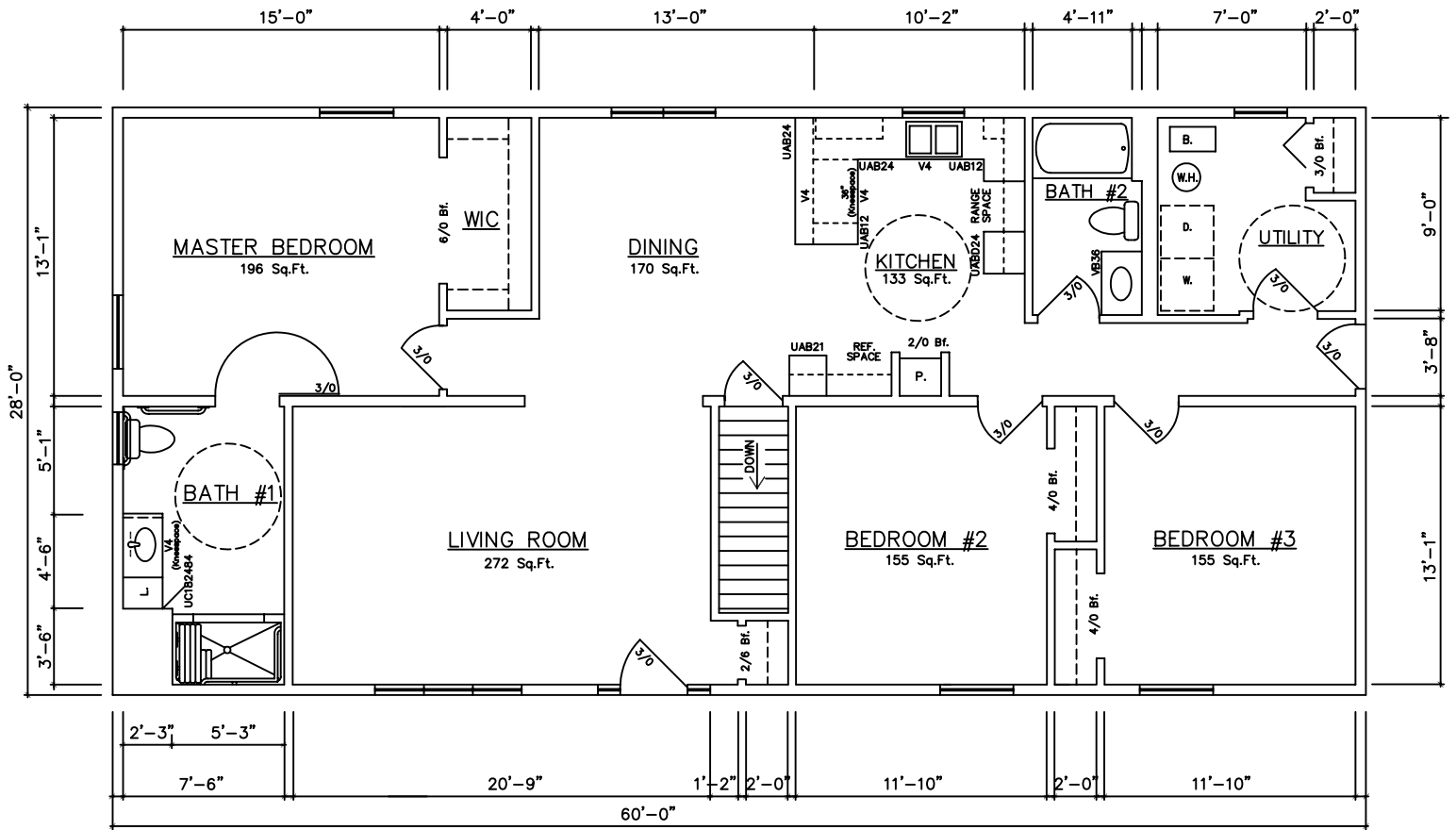
GROUND FLOOR PLAN (BASEMENT)
