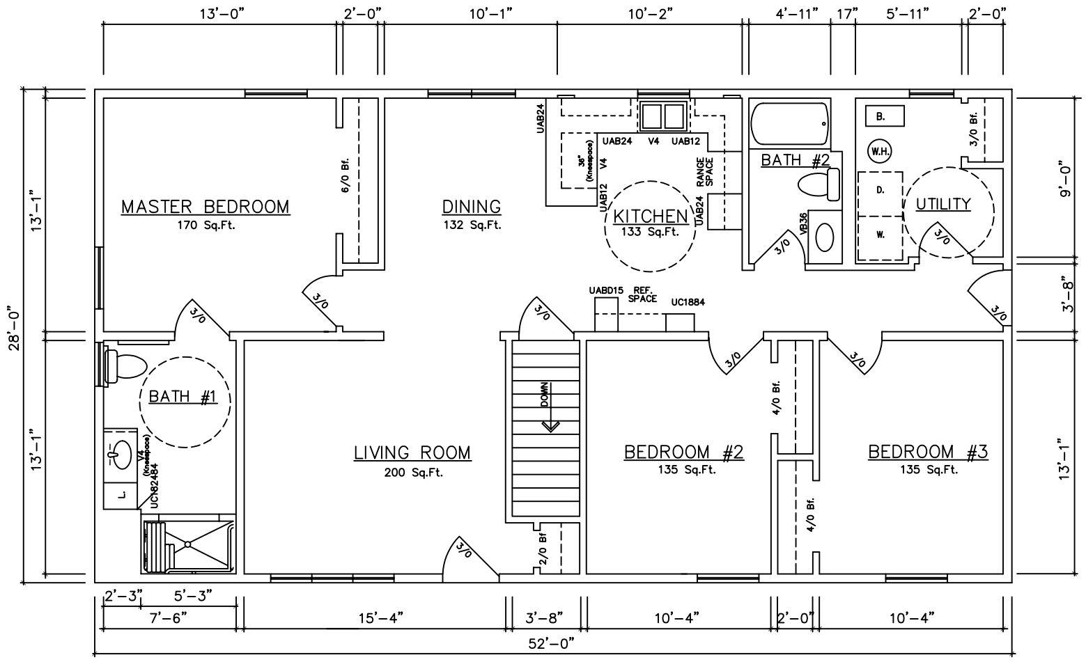
GROUND FLOOR PLAN (BASEMENT) LUDINGTON 28x52...12102UA
