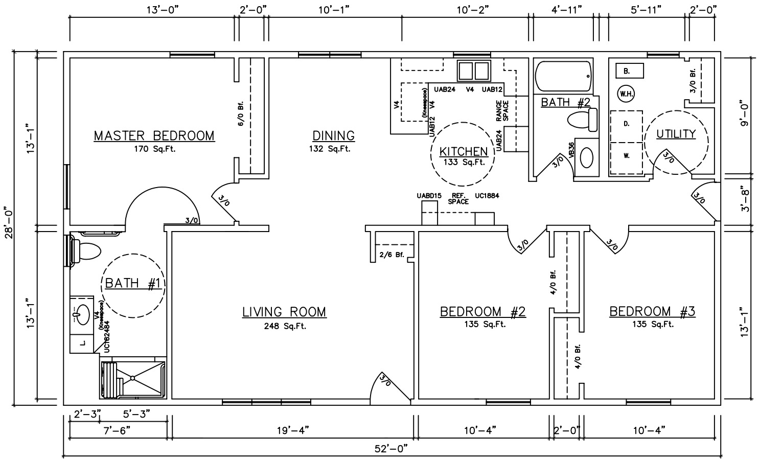
GROUND FLOOR PLAN (CRAWL)
