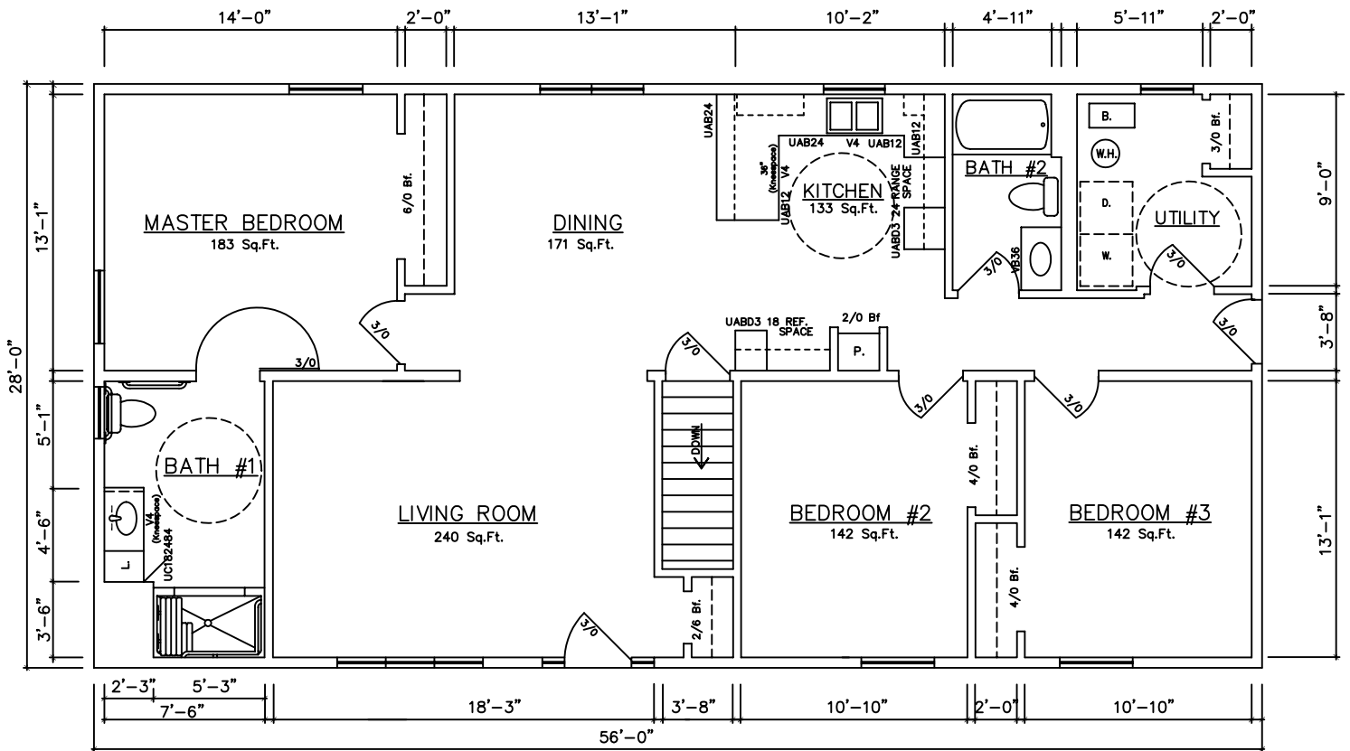
GROUND FLOOR PLAN (BASEMENT)
