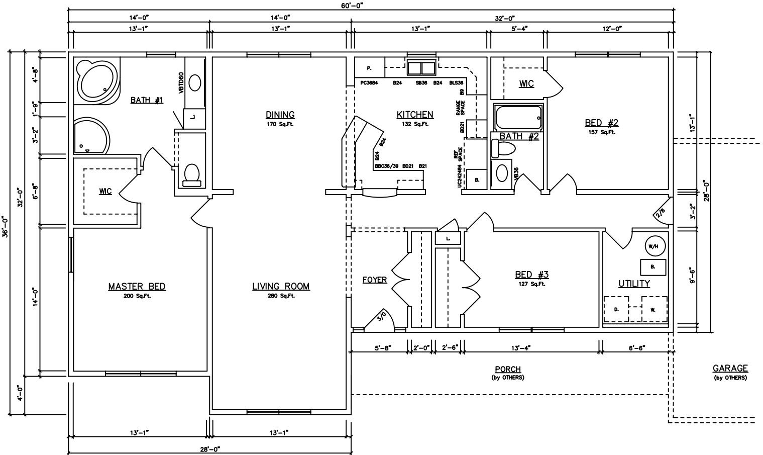
CRAWLSPACE FLOOR PLAN (End Load Garage) ESSEX II...14104 (1848 Sq.Ft.)
