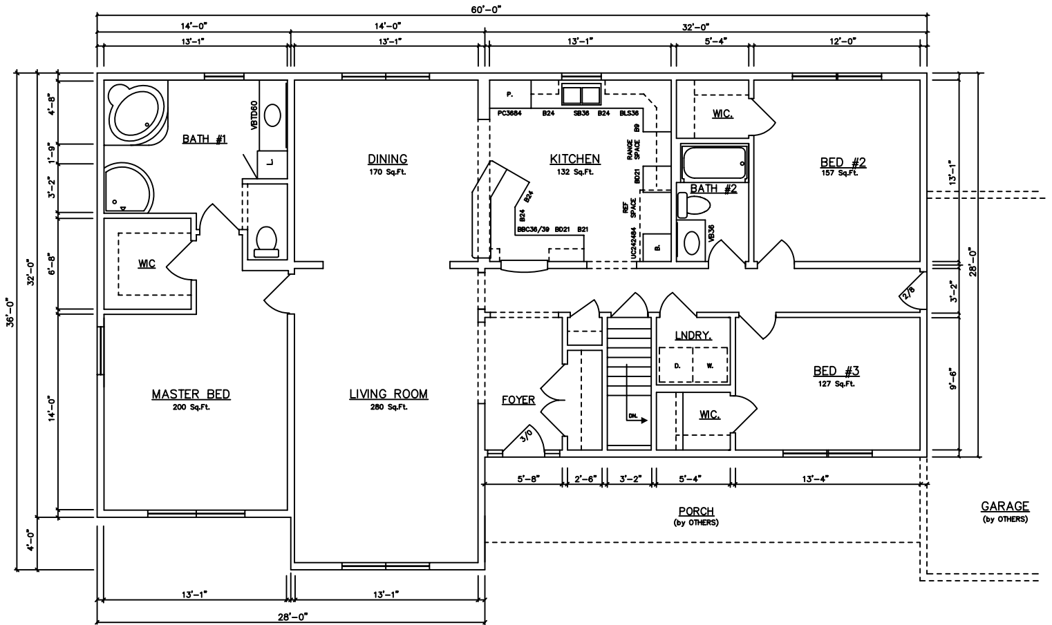
BASEMENT FLOOR PLAN (End Load Garage) ESSEX II...14106 (1848 Sq.Ft.)
