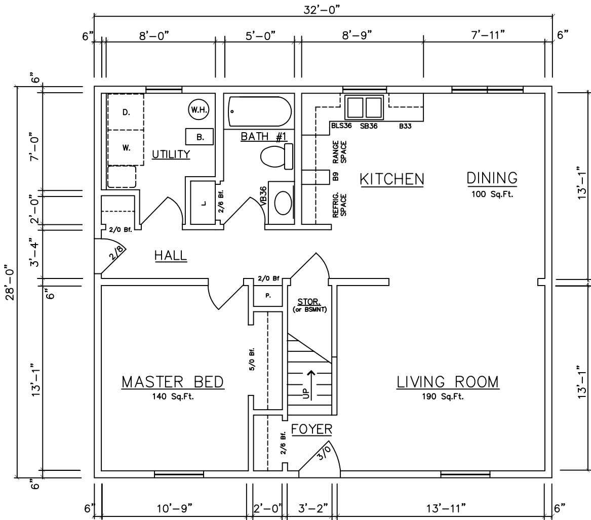
1st.FI. PLAN Williamsburg...11018 (CRAWLSPACE)
