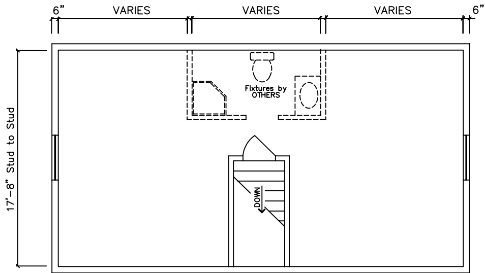
2nd.Fl. Plan
