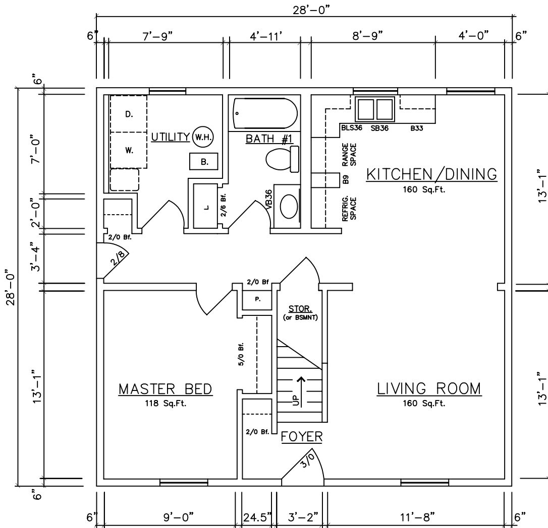
1st.Fl. PLAN Williamsburg .....11030 (CRAWLSPACE)
