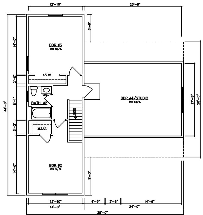
SECOND FLOOR PLAN 1056 Sq. Ft.
