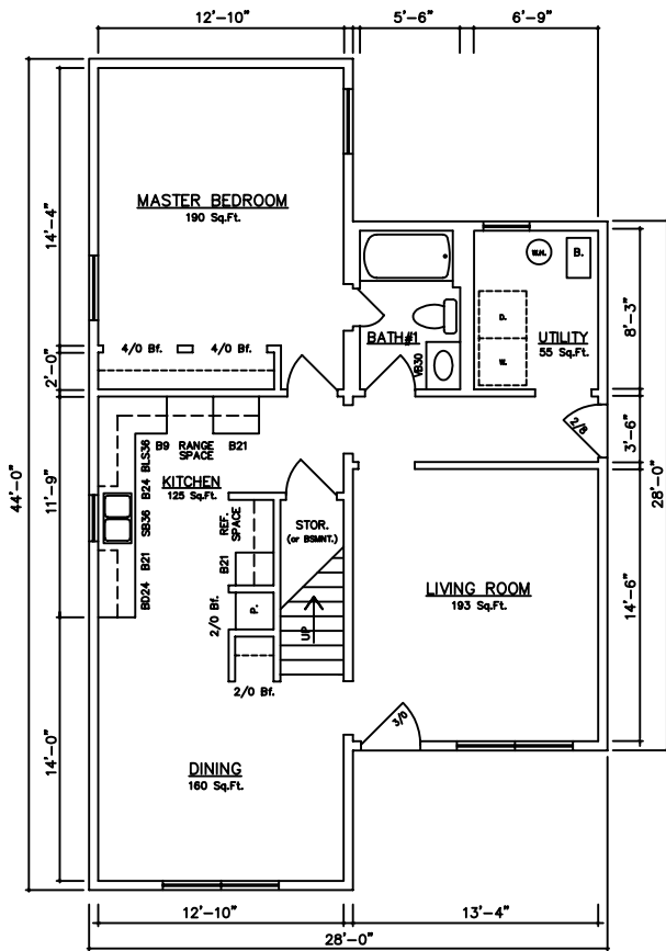
1st Floor BRECKENRIDGE 13116 (Basement) 13114 (Crawlspace)
