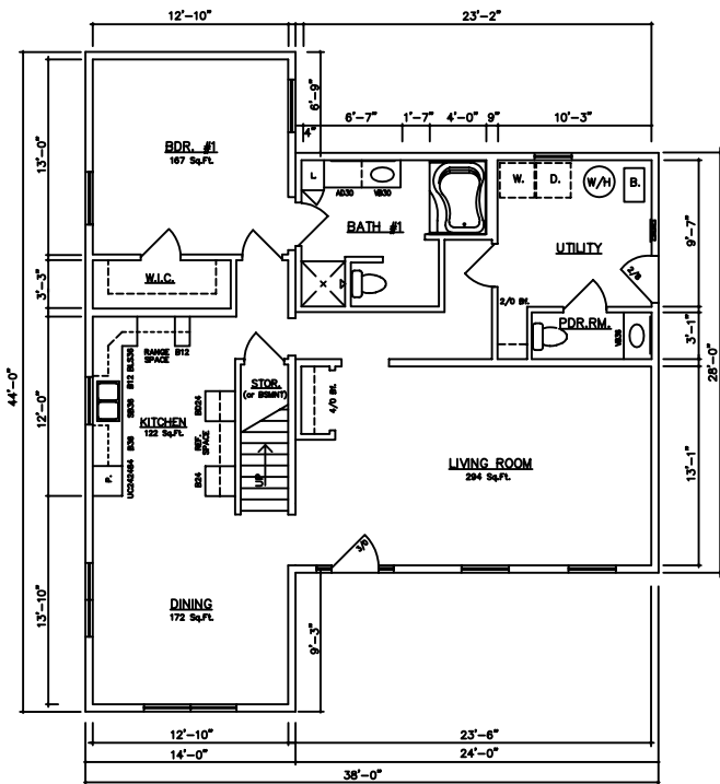
FIRST FLOOR PLAN 1288 Sq. Ft.
